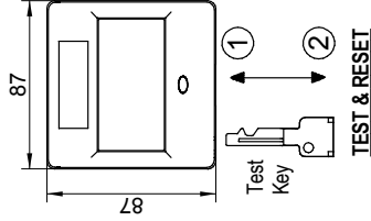
Fig.3 DIMENSIONS (mm)
